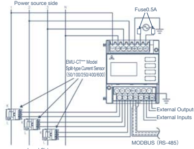
3P4W (For low-voltage circuit)
