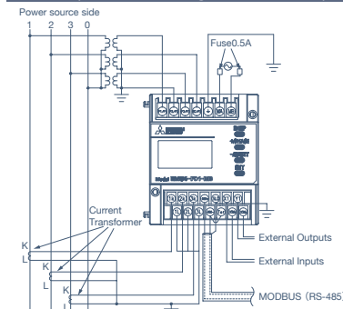
3P4W (with the voltage transformer)
